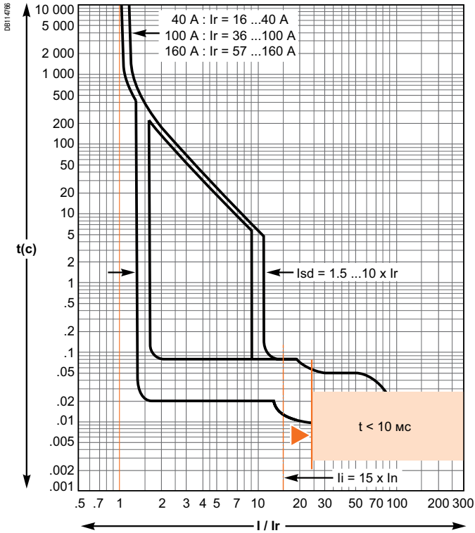
Micrologic 2.2 - 40... 160 A
