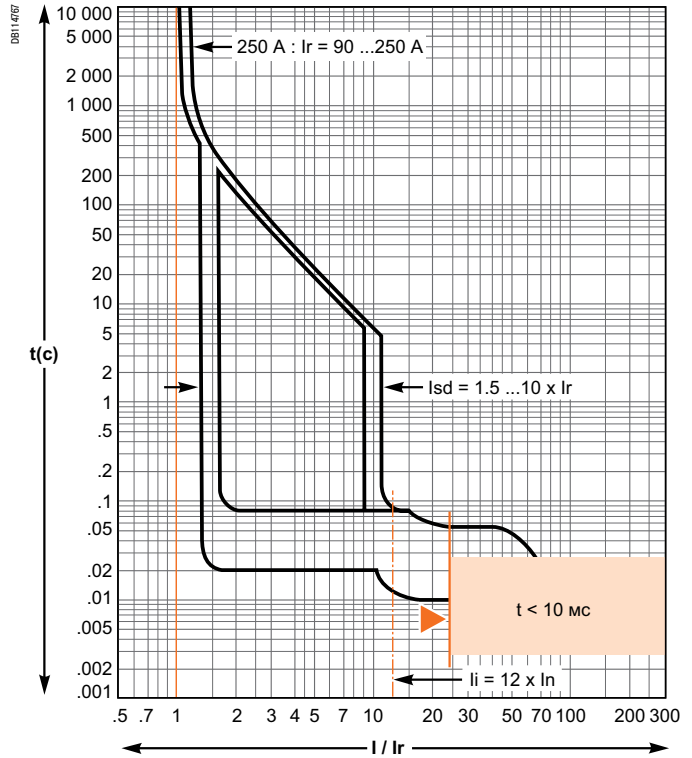
Micrologic 2.2 - 250 A
